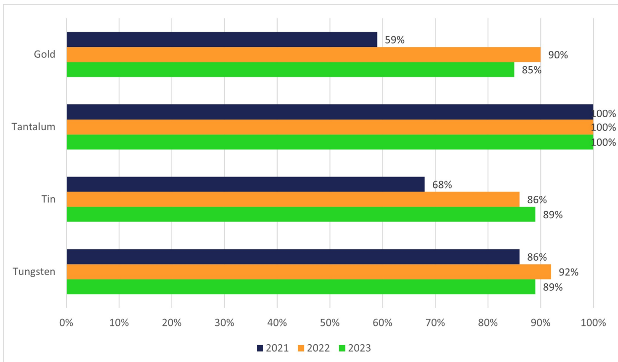
Figure 2: Three Year Comparison: Conformance % by Metal Type
